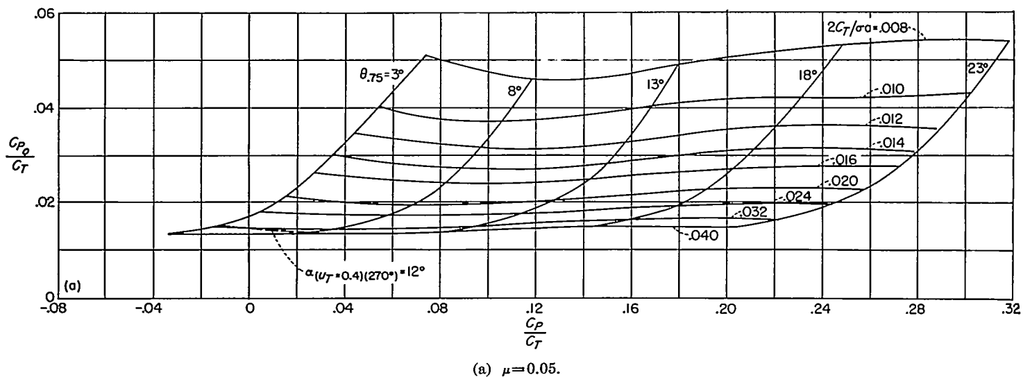
FIGURE 7.—Profile-drag—thrust ratio for blades having -16^\circ twist.
